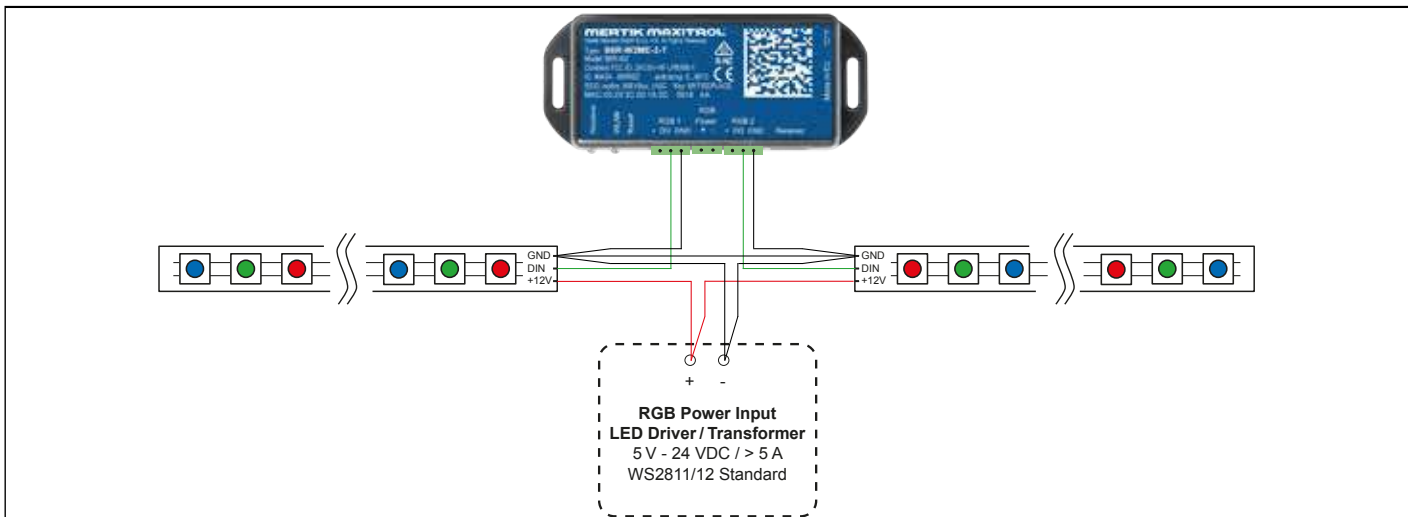
Figure 6: LED setup 2
