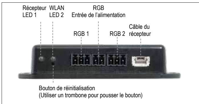
Figure 24: Wi-Fi Box (B6R-W2...)
