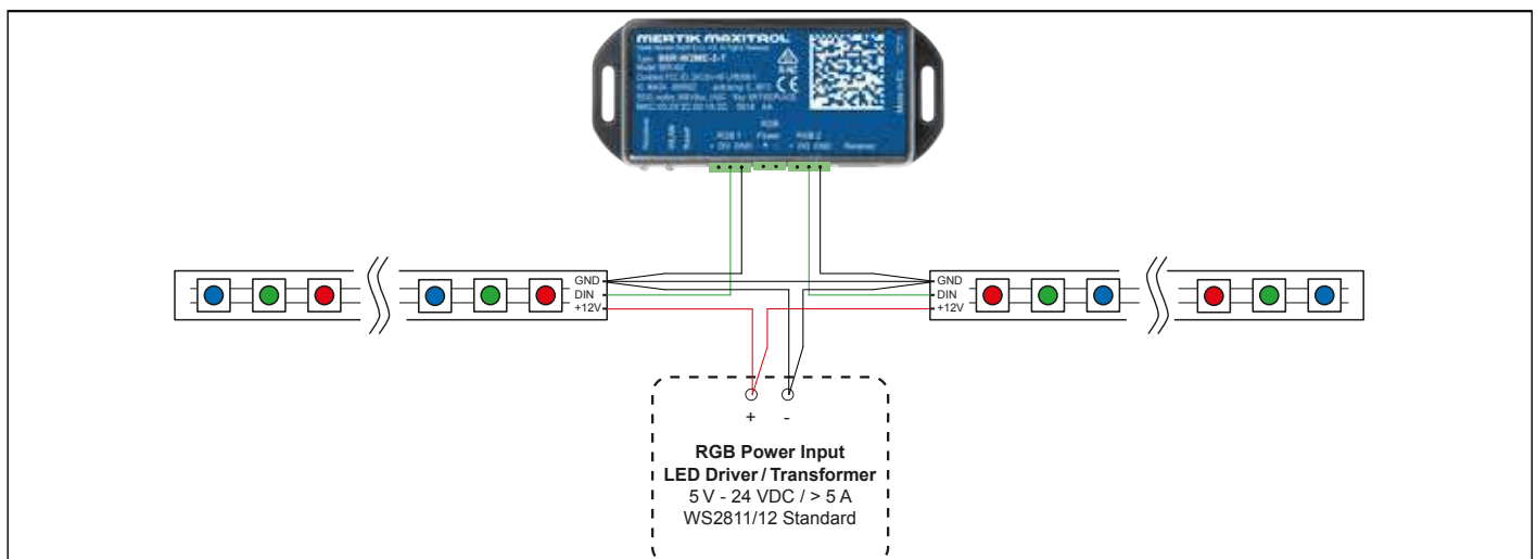
Abb. 5: LED setup 2
