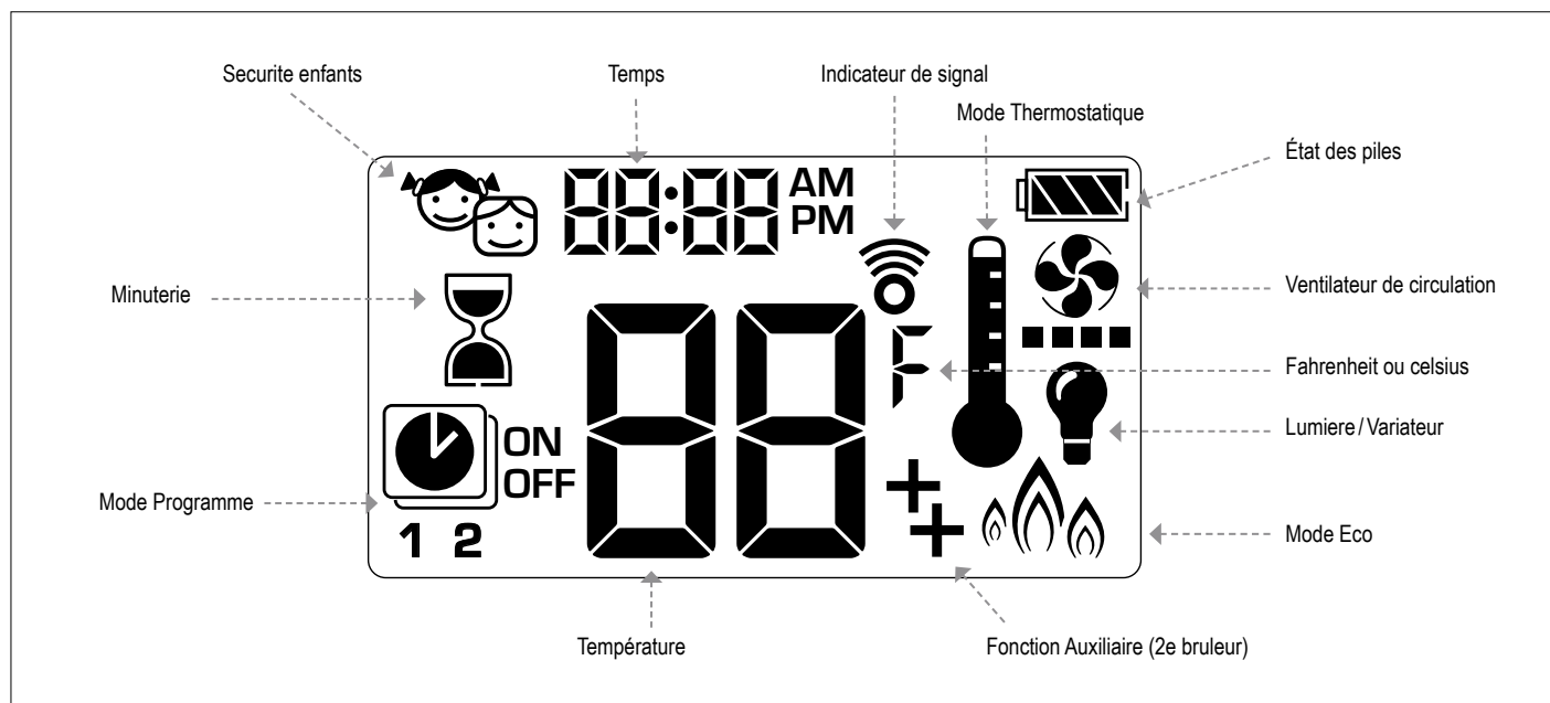
Figure 22: 10-symbol Display
