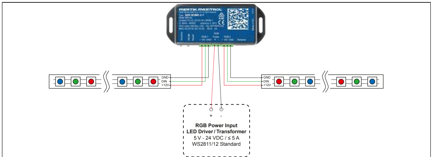
Abb. 4: LED setup 1
